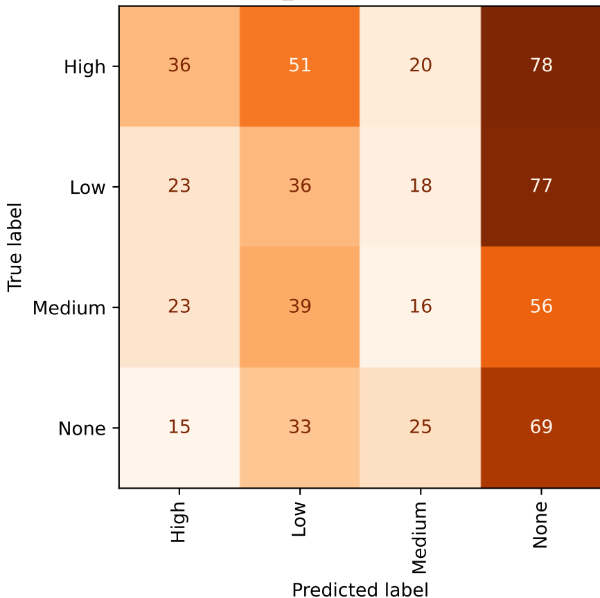
VLM — iq_imbalance (validation)
